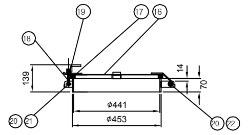
Man hole detail
