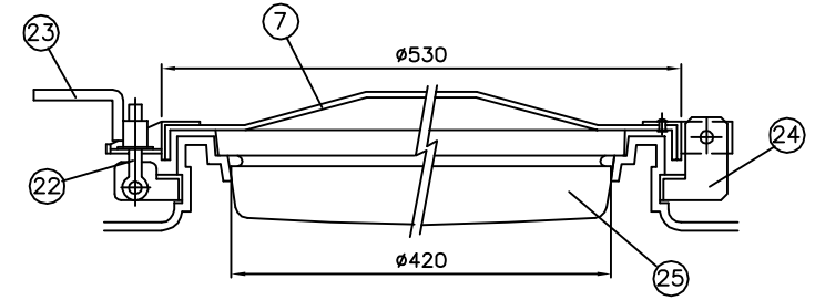
Manhole(M/H) ??? (1/5)
